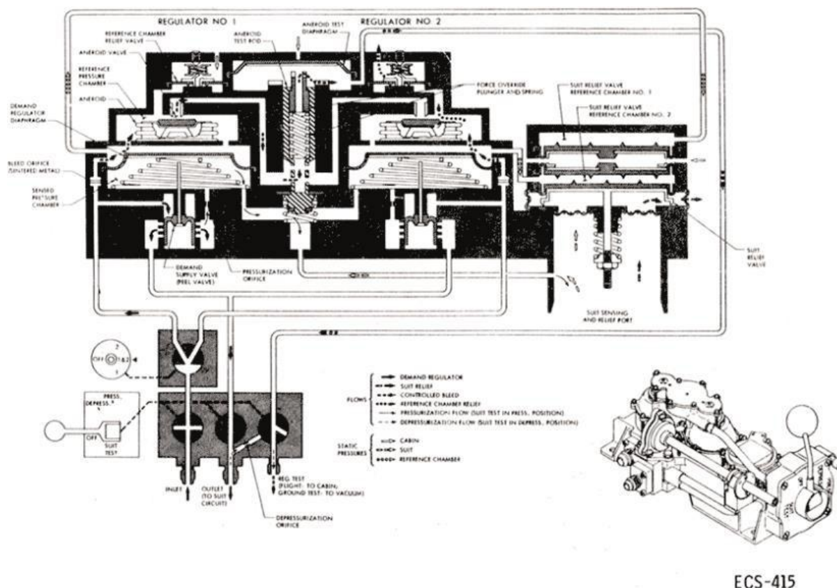
Figure 2.7-1. O 2 Demand Regulator
