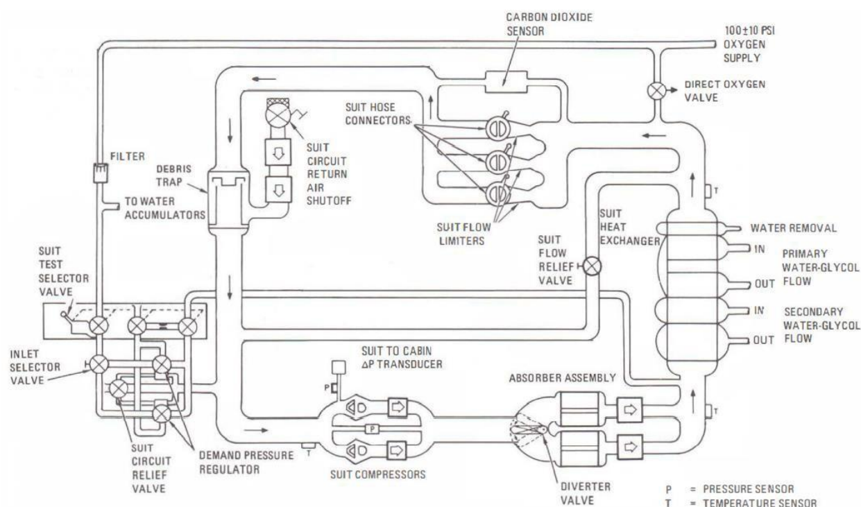
Simplified schematic of suit circuit
