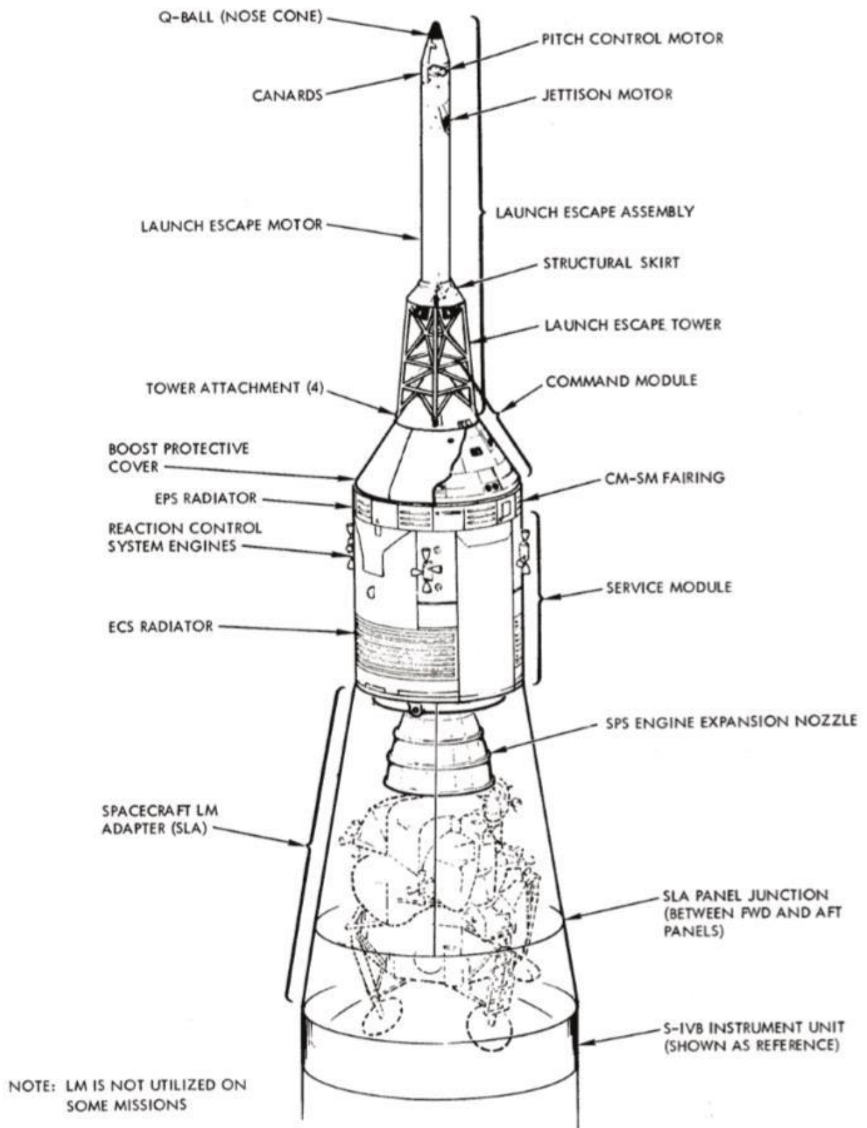
Figure 2.0.1 – The entire spacecraft
